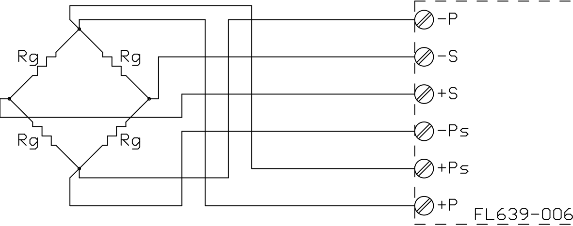
FULL BRIDGE CONFIGURATION
